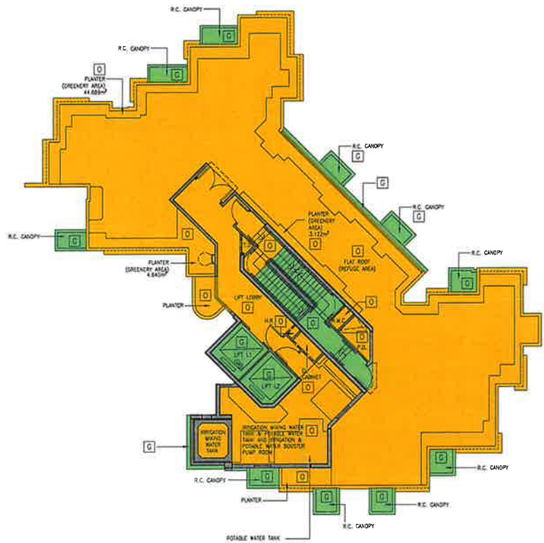
UPPER ROOF 2 FLOOR PLAN
