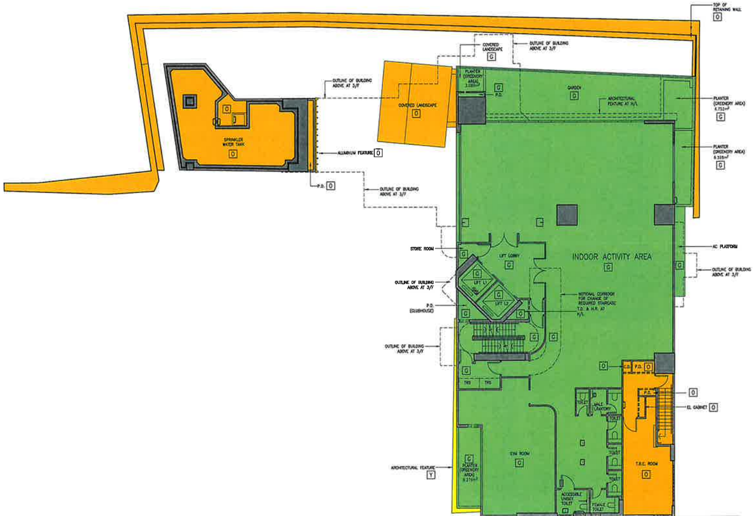
PART PLAN OF ST-1 & ST-2
