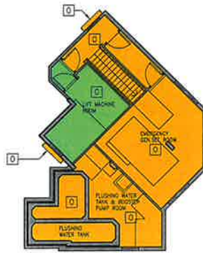
UPPER ROOF 2 FLOOR PLAN
