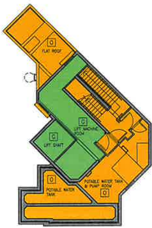
UPPER ROOF 1 FLOOR PLAN
